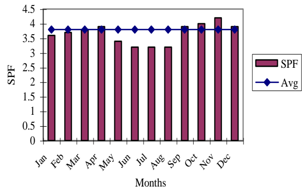
Figure 9: Seasonal performance for individual months and average for 2008.
