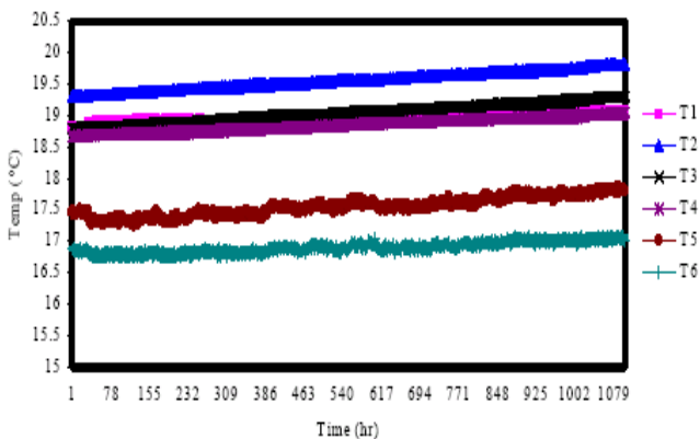
Figure 18: Variation of temperatures for heat exchanger for 45 days.
