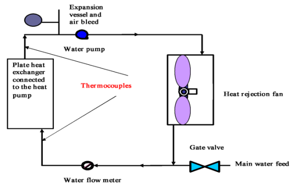
Figure 1: Sketch of installing heat pump
