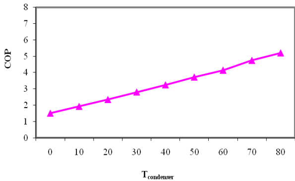
Figure 7: Heat pump performance vs condensation temperature
