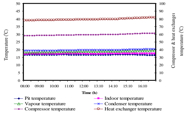
Figure 5: Variation of temperatures per day for the DX system. 2.3.1. Coefficient of Performance (COP)
