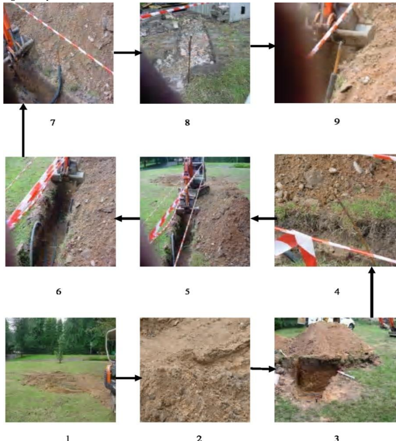
Figure 3: Showing the drilling (1-2) digging of the pit (3), connection of the manifolds (4), grouting, preparation of the coils (5-6) and the source loop, which consists of two earth loops: one for vapour and one for liquid (7-9).
