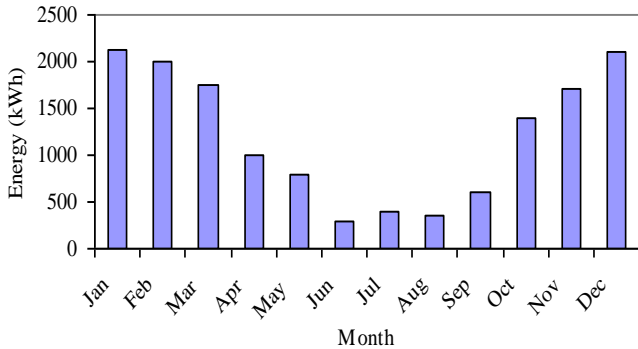
Figure 22: Monthly heating energy demands.
