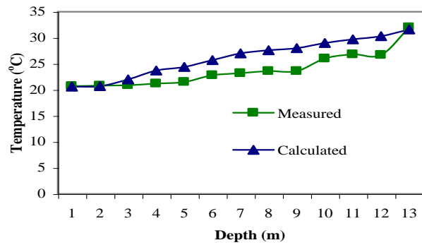
Figure 11: Comparison of calculations and experiments for saturated soil without groundwater flow (SS)
