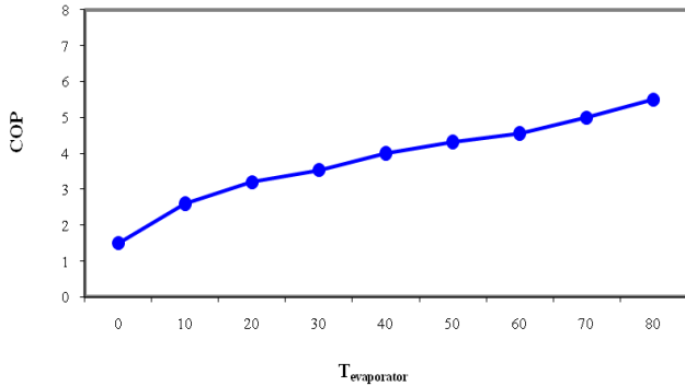
Figure 6: Heat pump performance vs evaporation temperature.
